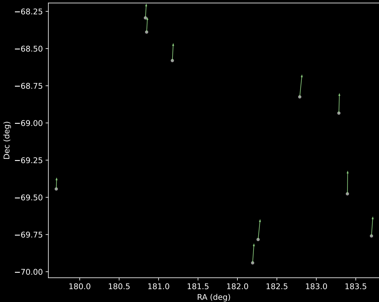
GALAH DR4 Cluster 5 Proper Motion Vectors (n=10)
