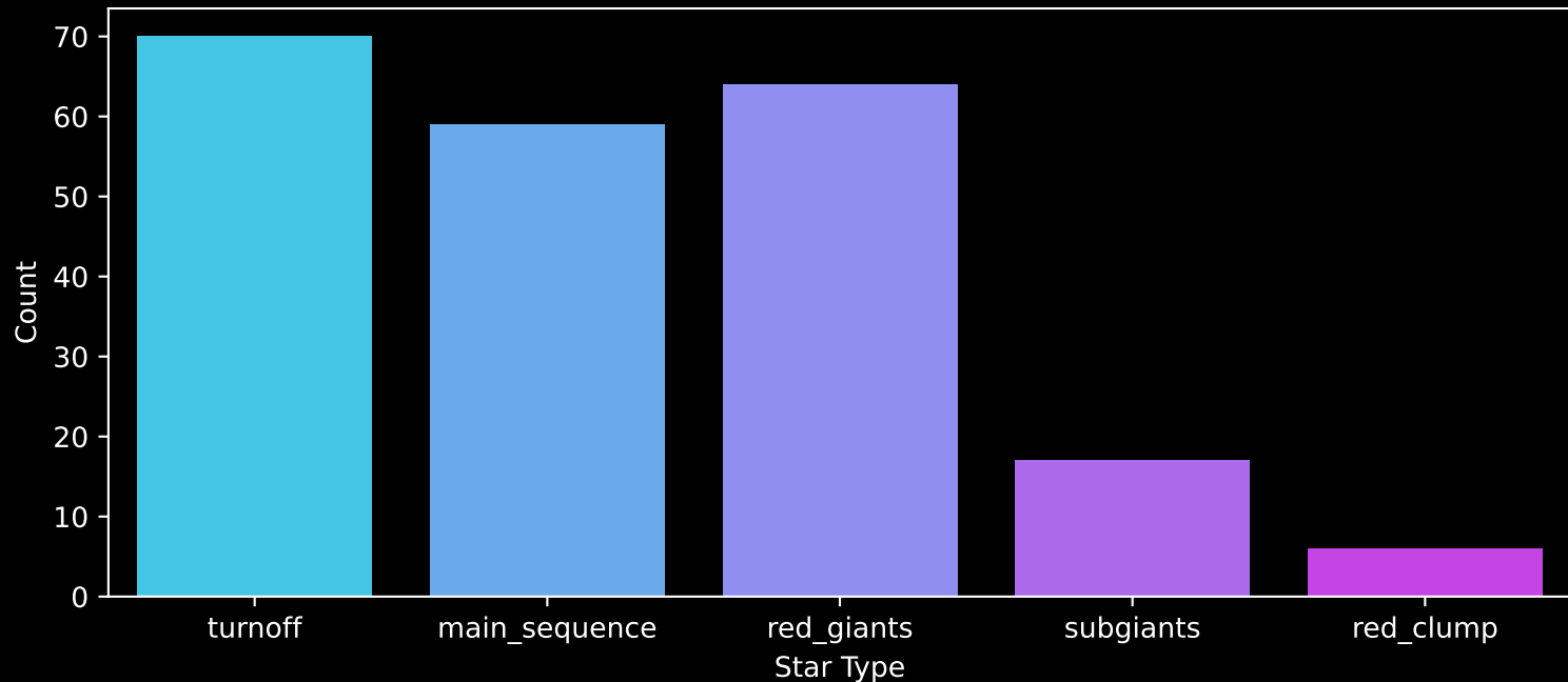
GALAH DR4 Field: [7135] Count plot of Star Type
