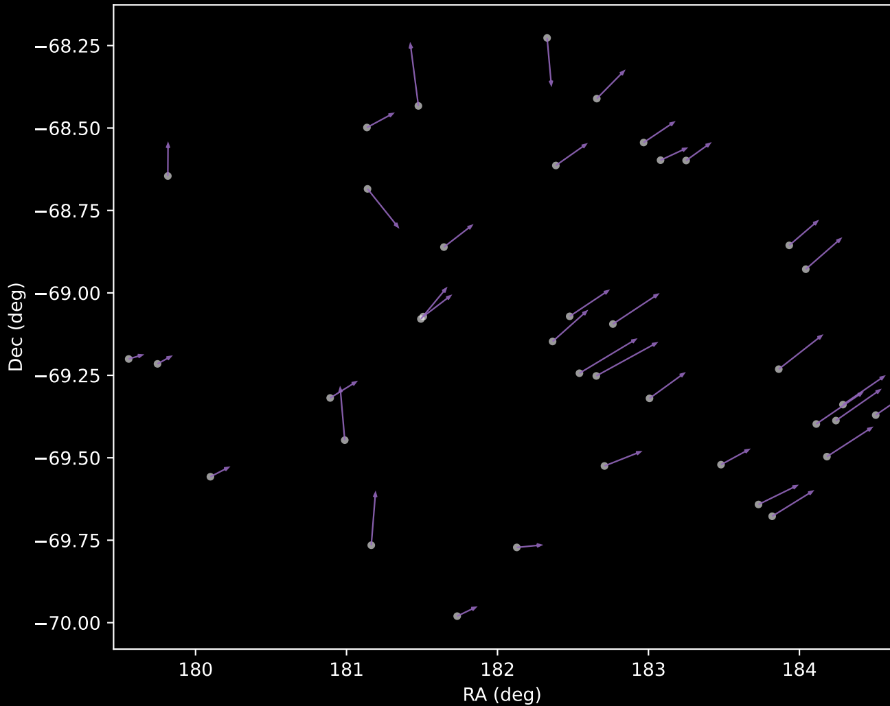
GALAH DR4 Cluster 8 Proper Motion Vectors (n=39)
