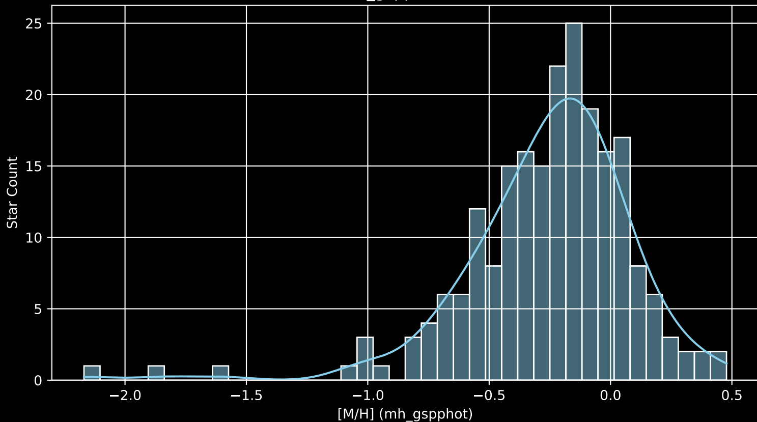
GALAH DR4 Field: [7135] [M/H] (mh_gspphot) (n= 215)
