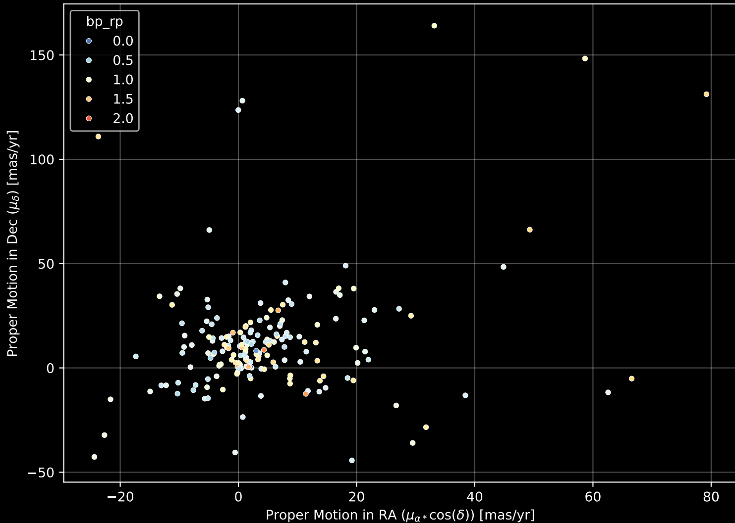
GALAH DR4 Field: [7135] Proper Motion Diagram (n= 216)
