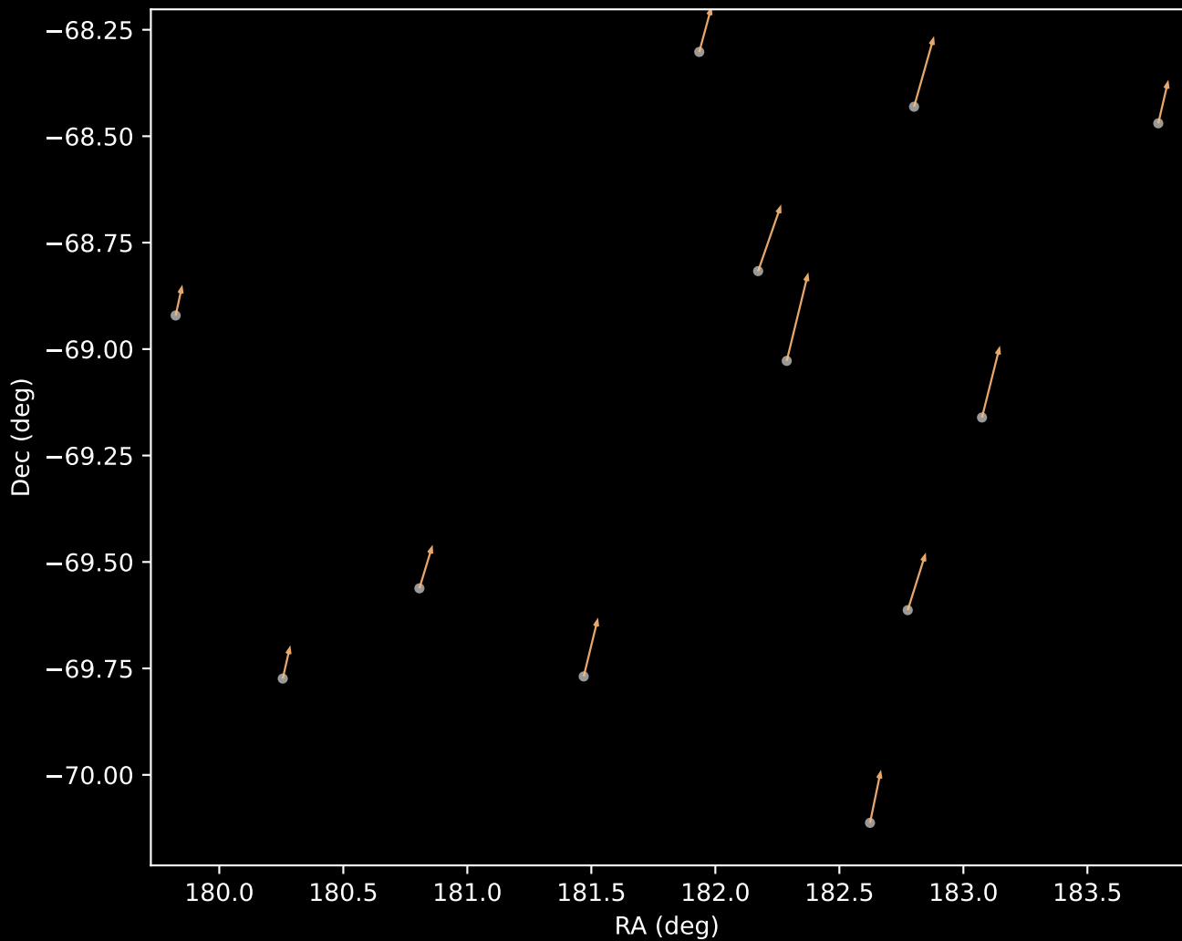
GALAH DR4 Cluster 3 Proper Motion Vectors (n=12)
