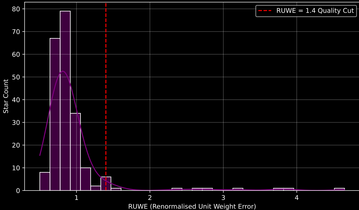
GALAH DR4 Field [7135] RUWE Distribution (n= 214)
